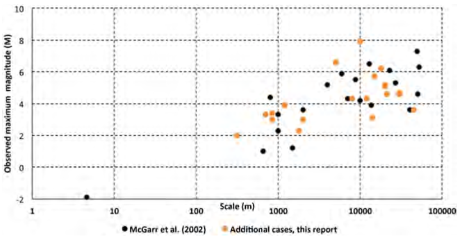
Fig. 102. M_{MAX} vs. project scale in meters. Black dots: cases studied by McGarr et al. (2002); orange dots: 20 additional cases from our database. Project scale was estimated using the longest dimension of the project, e.g., the length of a water reservoir.
