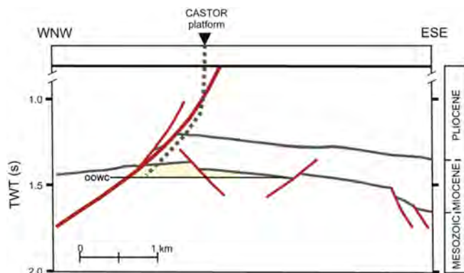
Fig. 74. Schematic diagram of the old Ampostá Oilfield, Spain, in WNW-ESE section. TWT: two-way travel time; dashed line: approximate location of the Castor injection well; OOWC: original oil-water contact at 1940 m depth; yellow area: approximate location of the gas reservoir. (From Gaite et al. (2016).)
