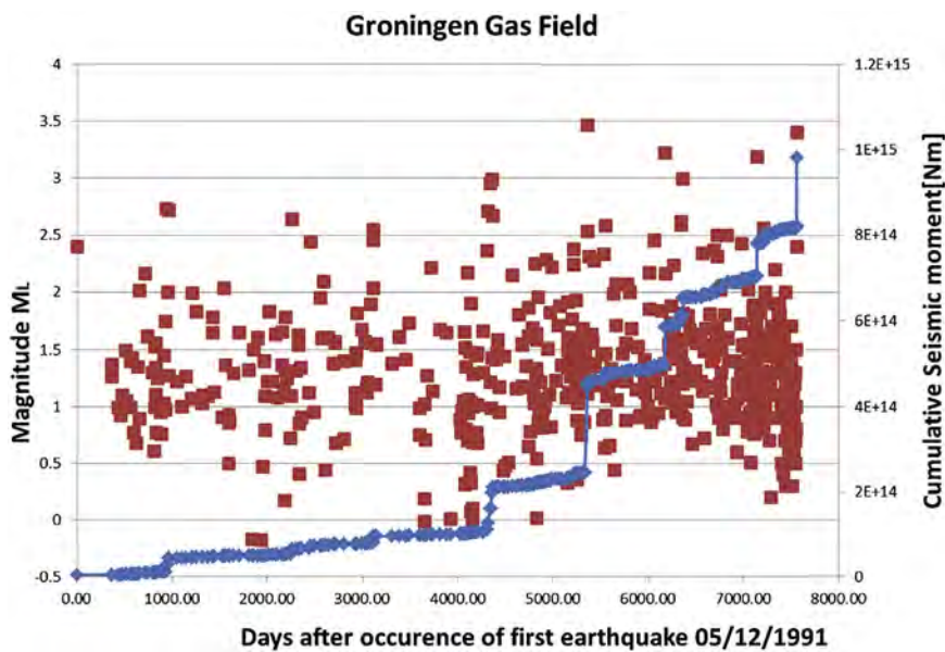
Fig. 32. Magnitude of induced events in the Groningen Gasfield, Netherlands, 5 December 1991–16 August 2012, and cumulative seismic moment in N m. (From Van Wees et al. (2014).)
